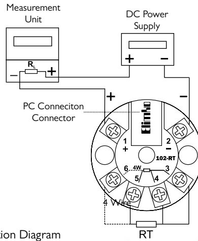
E-KC-102-R Connection Diagram
