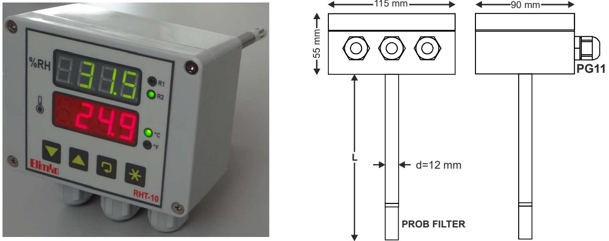
Figure 4.1. Overall Picture and Dimensions of E-RHT-10
